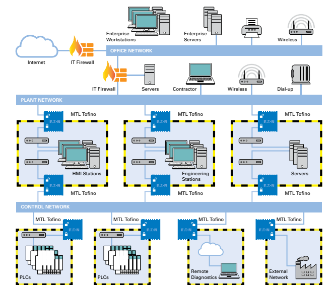
Zones and conduits provide defence in depth
