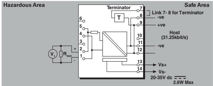
Test circuit for MTL5553
