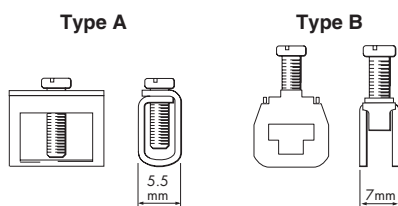
Figure 4.8: ETM7 Earth terminals
