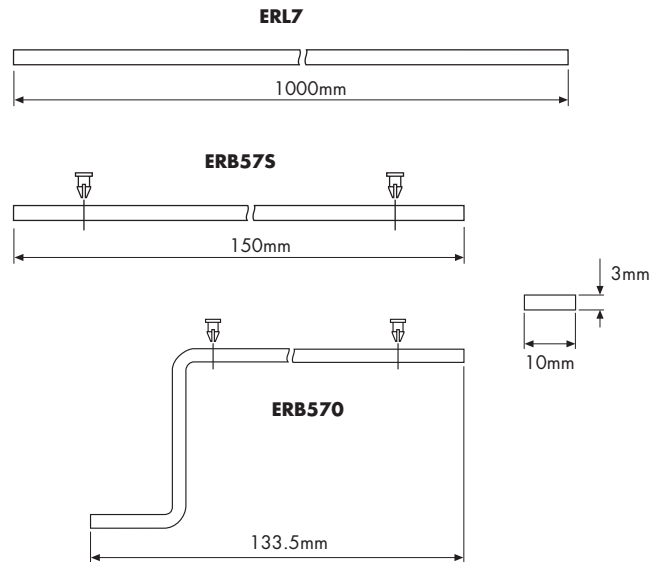
Figure 4.4: Mounting details
