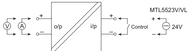
Figure 8.3: Powered DO test circuit
